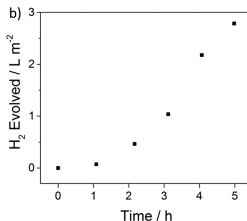
Fig. 9 (a) Side-view of the photoreactor set-up with reflective panel and polymer-coated glass fibers submerged in 5 vol% TEA and connected to a hydrogen collection vessel (right) (b) amount of hydrogen evolved over a 5 hour period on a largely overcast day (see supporting video of the experiment, ESI†).
