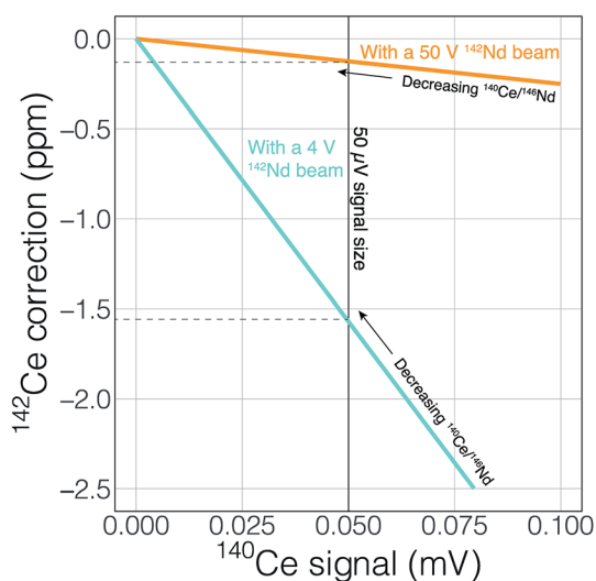
Fig. 10 The magnitude of correction for the isobaric interference of ^{140}\text{Ce} on the ^{142}\text{Nd} measurement as a function of the ^{140}\text{Ce} signal and varying Ce/Nd ratios. Two lines are shown, one with a 50 V ^{142}\text{Nd} beam and the other with a 4 V beam. All calculations were made assuming measurement on a Faraday cup and amplifier equipped with a 10^{11} \Omega resistor. A larger Nd signal will allow for more precise detection and application of important interferences, even if such interferences are not reduced. The same logic and calculations can be applied to many different types of analyses.
