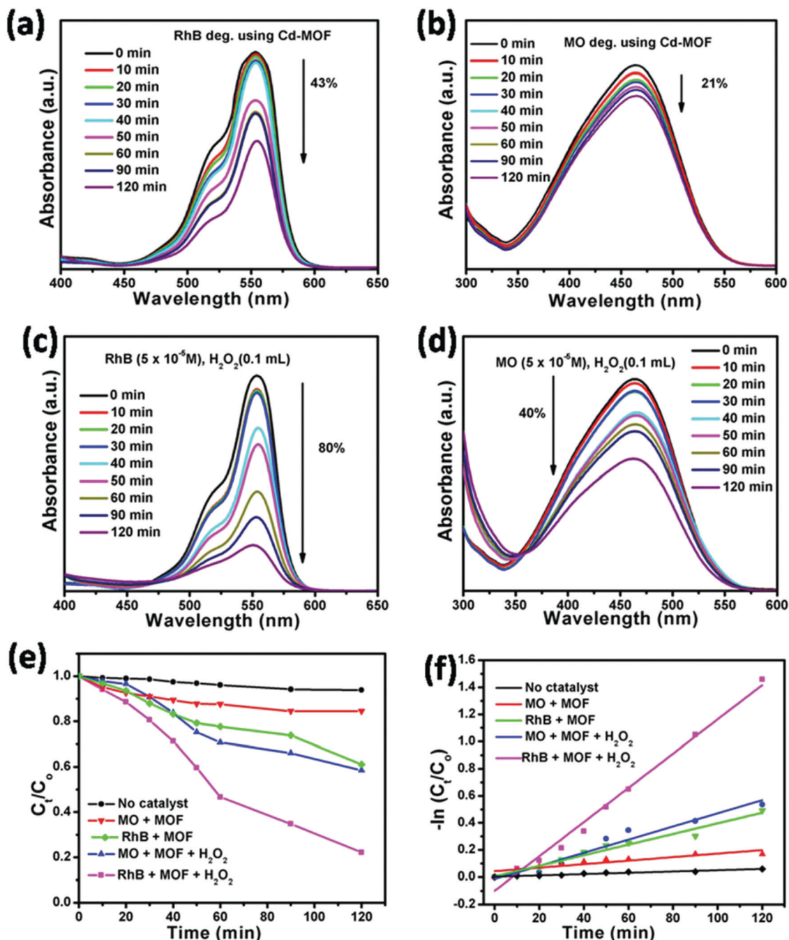
Fig. 18 UV-vis spectra for the photocatalytic degradation of RhB and MO (a) and (b) over Cd-MOF and (c) and (d) with the addition of H_2O_2 . Kinetic plots for the photocatalytic degradation of RhB and MO under various parameters (e) and (f). Reproduced from ref. 269 with permission from the Royal Society of Chemistry.
