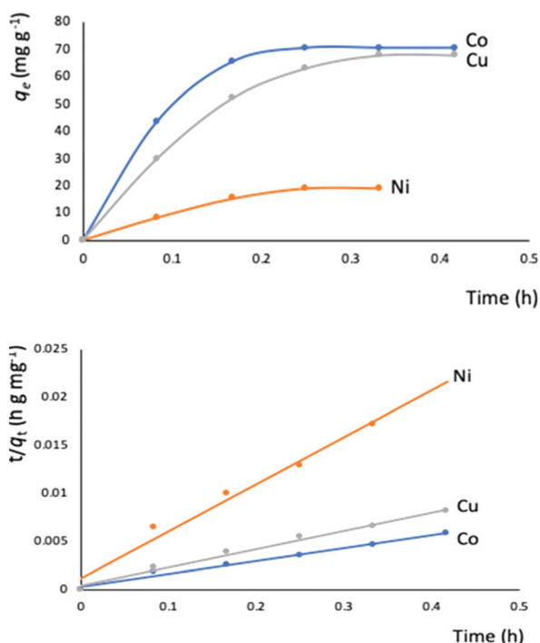
Fig. 7 Top: Metal adsorption capacity (mg g -1 ) versus time (h) plot. The solid lines is a guide to the eye; bottom: simulation of the experimental data to the pseudo-second order kinetic model. The solid lines represent the fitting of the data.
