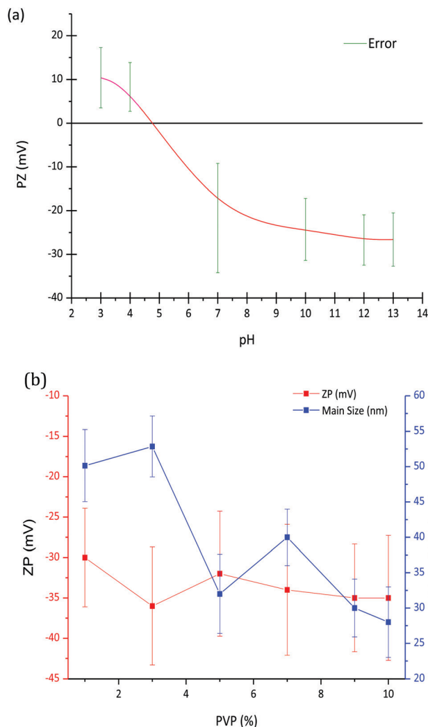
Fig. 1 (a) Variation of the ZP (mV) of \text{LaF}_3 -0.04 M nanoparticle suspensions as a function of pH and (b) variation of the zeta potential and particle size of \text{LaF}_3 -0.04 M nanoparticle suspensions at pH = 7 as a function of PVP wt%.
