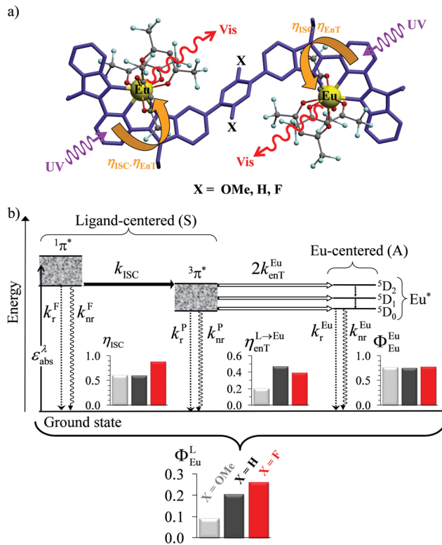
Fig. 6 (a) Molecular structures and (b) simplified Jablonski diagram for [(\text{hfac})_3\text{Eu}(\text{L})_2(\text{hfac})_3] showing the indirect ligand-centred triplet-mediated sensitization mechanism of the two \text{Eu}^{3+} activators. The photophysical processes are described by first-order rate constants: k_r^{\text{F}} = ligand fluorescence, k_{\text{nr}}^{\text{F}} = ligand internal non-radiative conversion, k_r^{\text{P}} = ligand phosphorescence, k_{\text{nr}}^{\text{P}} = non-radiative relaxation from the ligand triplet state, k_r^{\text{Eu}} = emission of \text{Eu}^* , k_{\text{nr}}^{\text{Eu}} = nonradiative decay of \text{Eu}^* , k_{\text{ISC}}^{\text{L}} = ligand intersystem crossing, and k_{\text{en.tr.}}^{\text{L} \rightarrow \text{Eu}} = ligand-to-metal energy transfer. Efficiencies of intersystem crossing ( \eta_{\text{ISC}} ), of energy transfer ( \eta_{\text{en.tr.}}^{\text{L} \rightarrow \text{Eu}} ), of intrinsic quantum yield ( \Phi_{\text{Eu}}^{\text{Eu}} ), and global quantum yield ( \Phi_{\text{Eu}}^{\text{L}} ) characterize the antenna effect (solid-state, 293 K). Adapted from ref. 17b.
