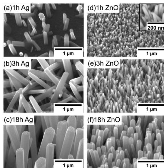
Fig. 5 ZnO NWs grown as a function of different times (45° tilted, temperature of 90 °C, precursor concentration of 40 mM), on Ag: (a) 1 hour, (b) 3 hours, and (c) 18 hours; on ZnO: (d) 1 hour with the high magnification image in the inset, (e) 3 hours, and (f) 18 hours.
