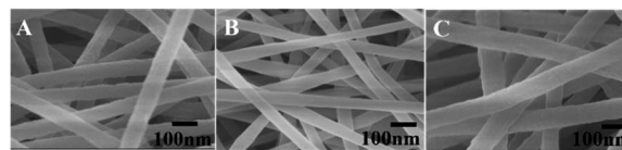
Fig. 1 SEM images of electrospun nanofibers prepared using different fluorescent polyacetylene (4.6 wt%) and PAN (7.4 wt%) mixtures in DMF solvent: (A) L -PCMF; (B) D -PCMF; and (C) PMF for detailed electrospinning parameters, see Table S2.†
