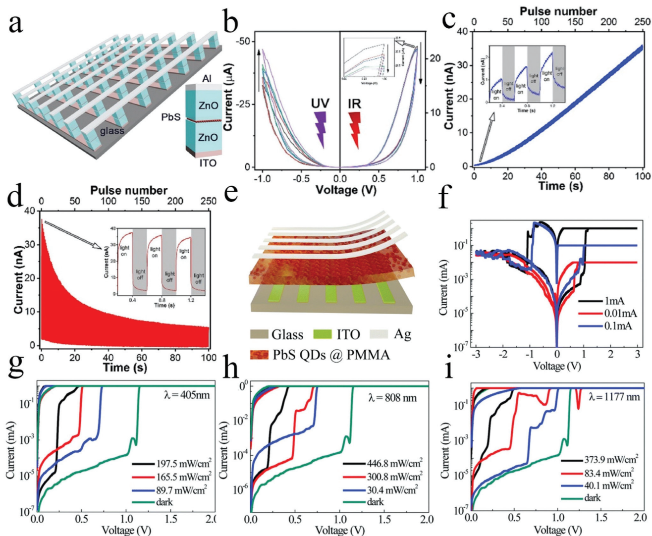
Fig. 6 (a) 3D schematic of the inorganic PbS/ZnO heterojunction-based memristor device array. (b) The I - V curves of the memristor device with UV and IR light irradiation. (c-d) The emulation of EPSC plasticity and IPSC plasticity by stimulation with 365 nm light pulses and 980 nm light pulses, respectively (light pulse: duration 0.2 s, interval 0.2 s). Reproduced with permission. 100 Copyright 2020, Elsevier. (e) The 3D device structure of the PbS QDs and PMMA composite film-based RRAM device. (f) Typical I - V curves of the RRAM device at various compliance currents. (g-h) Typical I - V curves of the RRAM device in the dark and with irradiation at different wavelengths. Reproduced with permission. 101 Copyright 2017, Royal Society of Chemistry.
