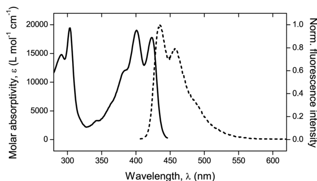
Fig. 3 UV-vis absorption spectrum (solid line) and normalized fluorescence emission spectrum (dashed line). \lambda_{exc} = 372 \text{ nm} .
