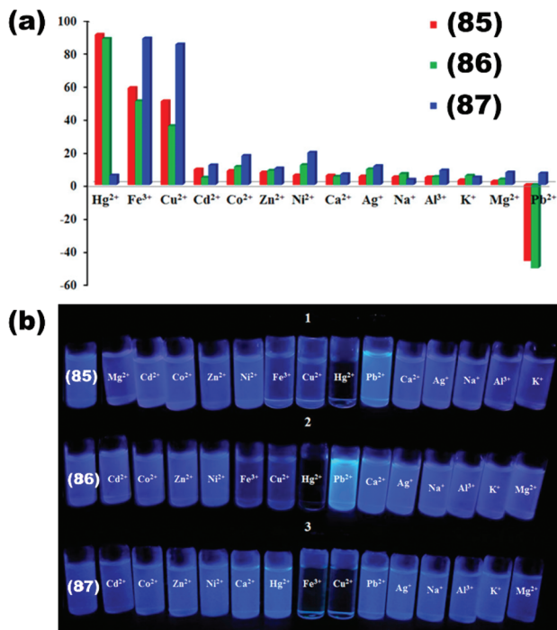
Fig. 12 (a) Quenching percentage of (85–87) in the presence of different metal ion solutions, (b) digital images (85–87) and after addition of different metal ion solutions under UV light (310 nm). Reproduced with permission from ref. 126. Copyright 2018 American Chemical Society.
