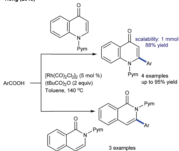
Scheme 12 C2-Arylation of quinolones/isoquinolones.
