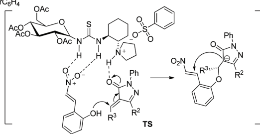
Scheme 32 Oxa-Michael/Michael cascade reaction for the synthesis of chiral spiro benzohydropyran-pyrazolones.
