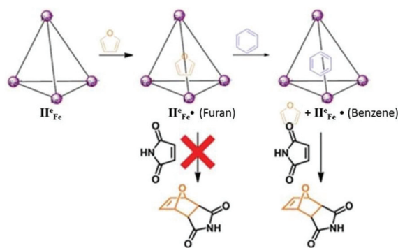
Fig. 26 Representation of trapping of furan by cage \text{II}_{\text{Fe}}^{\text{e}} , preventing it from undergoing a Diels-Alder reaction and the release of furan and initiation of a Diels-Alder reaction upon the addition of competing guest benzene. Reproduced with permission from ref. 95. Copyright 2012, Royal Society of Chemistry.
