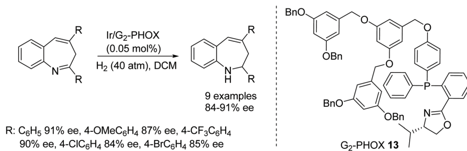
Fig. 18 Chemoselective and enantioselective AH of 2,4-diaryl-3H-benzobenzazepines.
