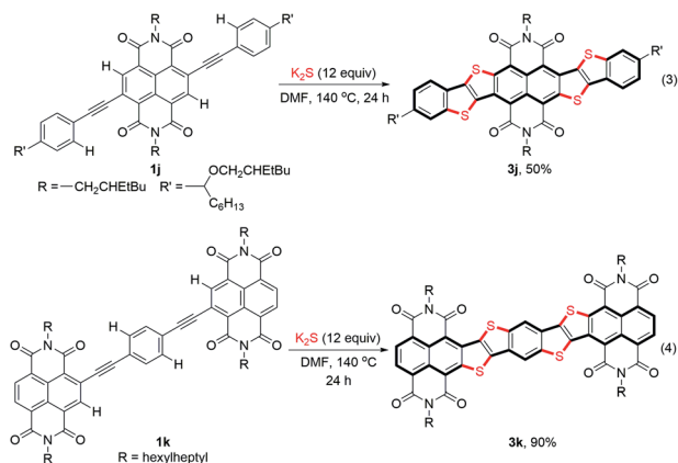
Scheme 3 Stitching thienannulations of 1j and 1k .
