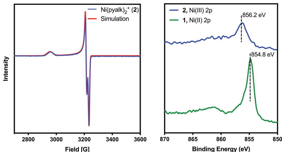
Fig. 2 (Left) Experimental (blue) and simulated (red) EPR spectra of 2 taken in \text{CH}_2\text{Cl}_2/\text{toluene} at 77 K. (Right) XPS spectrum of 2 (top) and 1 (bottom). The ~1 eV shift is consistent with a one-electron oxidation of the nickel center.
