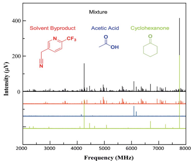
Fig. 4 Lower-temperature (120–130 °C) spectrum of the arylation product mixture. The strongest line is due to the cyclohexanone reagent. Weaker lines are due to the solvent-derived byproduct. The arylation reaction products are also present at lower levels.
