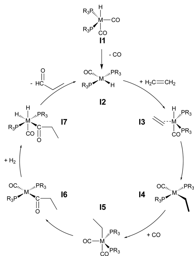
Scheme 2 Catalytic cycle depicting key intermediates for olefin hydroformylation by a transition metal catalyst.
