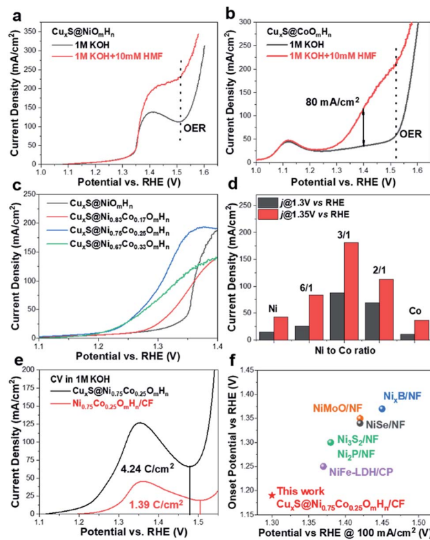
Fig. 2 (a and b) LSV curves of \text{Cu}_x\text{S}@\text{NiO}_m\text{H}_n and \text{Cu}_x\text{S}@\text{CoO}_m\text{H}_n towards electrochemical HMF oxidation. (c) Comparison of LSV curves of \text{Cu}_x\text{S}@\text{NiCo} LDHs with various Ni to Co ratios. (d) Current densities of prepared electrodes at 1.3 V and 1.35 V vs. RHE. (e) CV curves of \text{Cu}_x\text{S}@\text{Ni}_{0.75}\text{Co}_{0.25}\text{O}_m\text{H}_n , \text{Ni}_{0.75}\text{Co}_{0.25}\text{O}_m\text{H}_n/\text{CF} in 1 M KOH and calculated charges for the oxidation of transition metal cations prior to the oxygen evolution reaction. (f) Performance comparison of \text{Cu}_x\text{S}@\text{Ni}_{0.75}\text{Co}_{0.25}\text{O}_m\text{H}_n/\text{CF} with reported electrocatalysts towards electrochemical oxidation of HMF, urea and primary amine.
