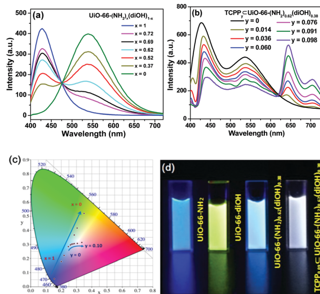
Fig. 2 Photoluminescence spectra of the suspensions of (a) \text{UiO-66-(NH}_2)_x(\text{diOH})_{1-x} and (b) \text{TCPP}_y\text{-UiO-66-(NH}_2)_x(\text{diOH})_{1-x} . (c) CIE chromaticity diagram for the MOF samples. (d) Photographs of MOF suspensions under UV lamp irradiation. 50 mg \text{L}^{-1} MOF in aqueous suspension, \lambda_{\text{ex}} = 388 nm.
