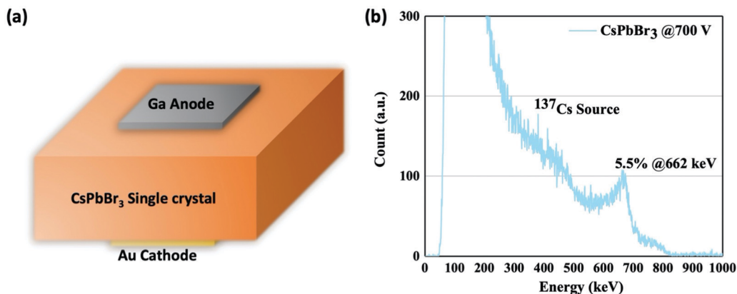
Fig. 4 (a) Schematic of detector structure (4.5 mm \times 4.5 mm electrode area, 2.5 mm thickness). (b) 662 keV 137 Cs spectrum acquired by CsPbBr 3 single crystal under 700 V.
