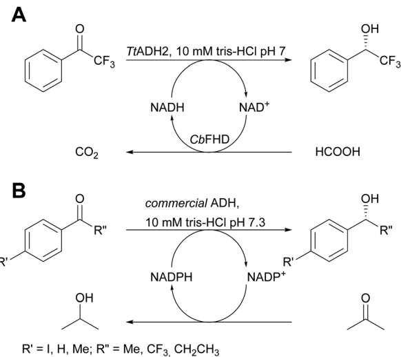
Scheme 2 (A) Asymmetric reduction of 2,2,2-trifluoro-1-phenylethan-1-one catalysed by TtADH2 with external cofactor recycling by CbFDH ; (B) asymmetric reduction of ketones with internal cofactor recycling.
