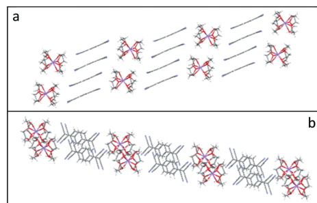
Fig. 8 Side (a) and top (b) views of the sheets of face-to-face \pi -stacked columns of TCNQ dimers formed in (12-crown-4) 2 Li(TCNQ) 2 ( 3 ), revealing the long-axis slipped character of the TCNQ dimer.
