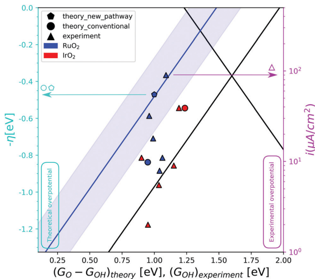
Fig. 2 The OER activity volcano. The red data points correspond to \text{IrO}_2 and the blue ones to \text{RuO}_2 . The triangles represent the experimental data in varying pH conditions, 27,28 while the circle and the pentagon are theoretical data for the conventional and the \text{RuO}_2 pathway respectively. The blue trend line corresponds to the strong binding side of the volcano if the \text{RuO}_2 pathway is followed. The blue shaded area around the blue trend line, is the DFT error of \pm 0.2 eV. The left y-axis (cyan) presents the theoretical overpotential and the right y-axis (magenta) presents the experimental overpotential, as the logarithm on the current is what you would expect from the Butler–Volmer equation to compare with potential. As we can only hope to compare trends, and not absolute numbers, the theoretical and experimental overpotentials are calibrated by overlapping the theoretical and experimental overpotential for \text{IrO}_2(110) . We cannot expect the scale of changes to be the same for calculations and experiments as the predicted differences are often larger than the measured. This figure is therefore two different figures overlapped for the comparison of trends. This also means that the two y-axes can be scaled and translated relative to each other. Two different descriptors with the same scale are used on the x-axis. G_{\text{O}} - G_{\text{HO}} and G_{\text{HO}} for the theoretical and the experimental data respectively.
