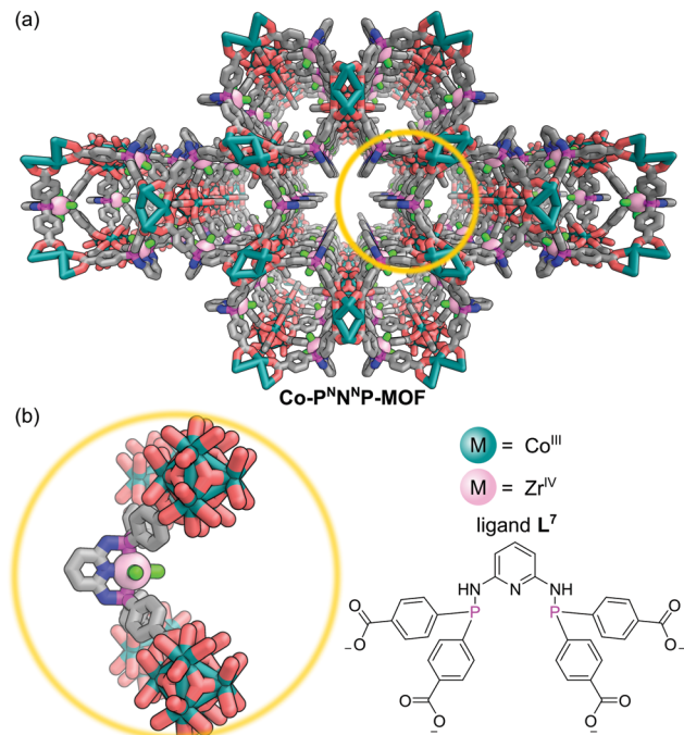
Fig. 10 (a) The 3D MOF formed by reaction of [Co(L^7)Cl_3] with ZrCl_4 exhibits an unusual csq topology in which Zr_6 clusters are linked through the P^{N^N^N}P pincer ligand; (b) the [Co(P^{N^N^N}P)Cl_3] complex is retained in the synthesis protruding into the MOF cavities. Hydrogen atoms omitted for clarity. Colours: C grey, Cl bright green, Co teal, N blue, O red, P magenta, Zr light pink (shown as spheres).
