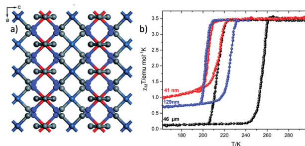
Fig. 2 (a) Grid-like layers of [Fe(py) 2 Ni(CN) 4 ] along the b axis; color code: Fe, red; Pt, turquoise; Ni, blue; N, green; C, grey; (b) the effect of downsizing of [Fe(py) 2 Ni(CN) 4 ] on the magnetic susceptibility. Adapted from ref. 28, licensed under CC BY 3.0, published by the Royal Society of Chemistry.
