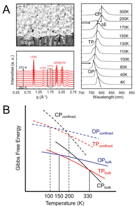
Fig. 9 (A) SEM image of MAPbI 3 confined within 100 nm diameter nanopores of anodized aluminium oxide templates. Temperature-dependent X-ray diffraction measurements revealed only the cubic phase to be present in the range of 293–373 K, while temperature-dependent photoluminescence measurements revealed the tetragonal (TP)–cubic (CP) phase transition to occur between 170–200 K and the orthorhombic (OP)–TP transition to occur between 80 and 100 K. (B) Comparison of the dependence of the Gibbs free energy on temperature for different polymorphs of a compound in the bulk and nanocrystal state. Reproduced with permission from ref. 130. Copyright 2019, American Chemical Society.
