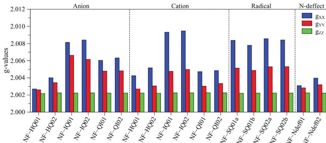
Fig. 4 DFT derived g -values for anionic, cationic and radical NF-melanin units. 01 and 02 refer to NF-DHI and NF-DHCA species, respectively.
