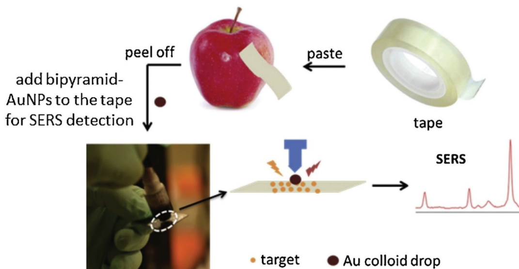
Fig. 4 Detection of pesticides using SERS substrates. The schematic shows the use of modified adhesive tape modified with bipyr amid-gold nanoparticles (AuNPs) as a SERS sensor for pesticide residue detection on the surface of fruit peels. Reproduced with permission from ref. 51. Copyright 2019, Elsevier.
