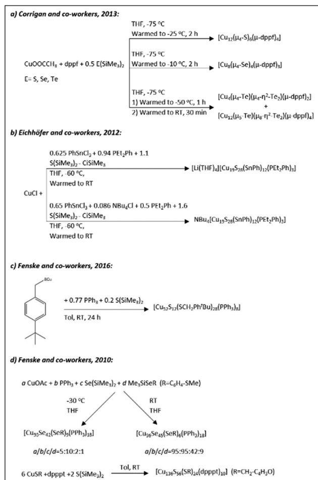
Scheme 2 The syntheses of chalcogen-bridged CuNCs as described in ref. 166 (Reprinted with permission, Copyright 2013 American Chemical Society), ref. 176 (Reprinted with permission, Copyright 2012 Royal Society of Chemistry), ref. 193 (Reprinted with permission, Copyright 2016 Royal Society of Chemistry), ref. 197 (Adapted with permission, Copyright 2010 Wiley-VCH Verlag GmbH & Co. KGaA, Weinheim).
