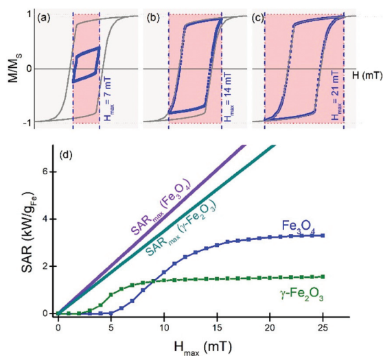
Fig. 2 Representative hysteresis loops for randomly dispersed non-interacting magnetite nanoparticles for different values of H_{\max} : (a) 7 mT, (b) 14 mT, and (c) 21 mT, for f = 765 kHz and T = 0 K. In each case the coloured rectangle stands for the maximum possible area, and the grey curve line corresponds to the theoretical quasistatic limit. Panel (d) shows the SAR vs. H_{\max} evolution of both pure magnetite ( \text{Fe}_3\text{O}_4 ) and maghemite ( \gamma\text{-Fe}_2\text{O}_3 ) cases for the same frequency and again without thermal effects, where the solid lines stand for the associated maximum possible value (square loop) based on the corresponding M_S values.
