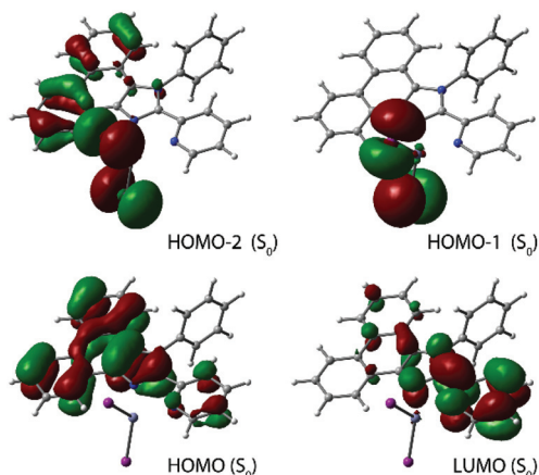
Fig. 3 Frontier molecular orbitals for the ground states of complex 11 (in chloroform, the singly occupied orbitals for S_1 and T_1 states are shown in Fig. S4†).
