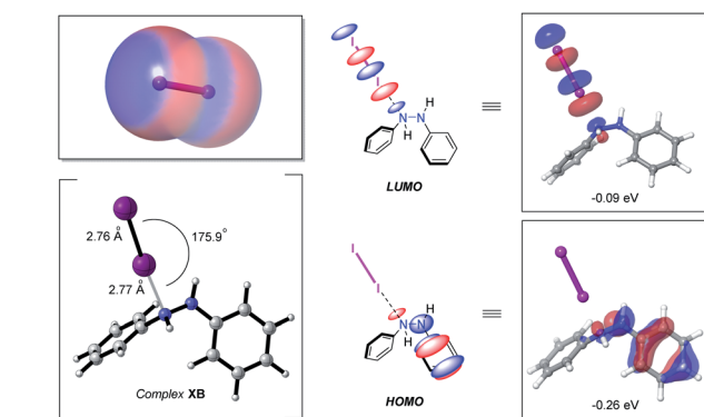
Fig. 2 Electrostatic potential surface of \text{I}_2 (electronegative (red) and electropositive (blue) regions (left-hand side, top)) computed at the B3LYP-D3/lacv3p**++ level of theory (isovalue = -0.003 (max = 0.3 , min = -0.3 )). Halogen bond complex XB (left-hand side, bottom) computed at the (IEFPCM DCM )UAPFD/def2-TZVP//UAPFD/DGDZVP level of theory. Chemdraw and computed HOMO and LUMO of complex XB with orbital energies in eV (middle and right-hand side).
