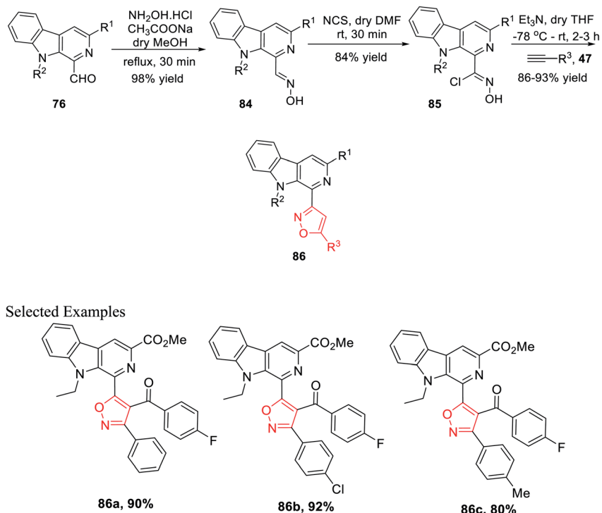
Scheme 20 Formation of the \beta -carboline-(C-3) isoxazole derivative via the oxime intermediate.
