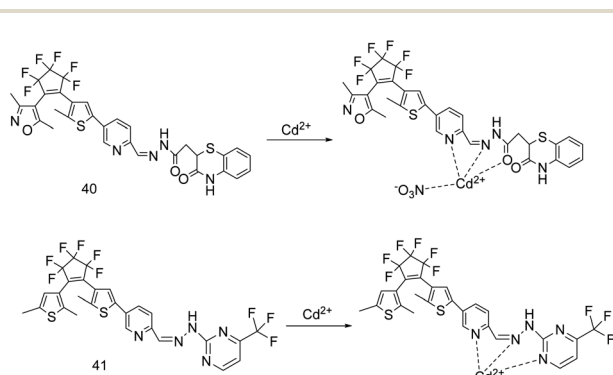
Fig. 14 The probes structure reported by Z. Wang's team and proposed binding mode with \text{Cd}^{2+} .
