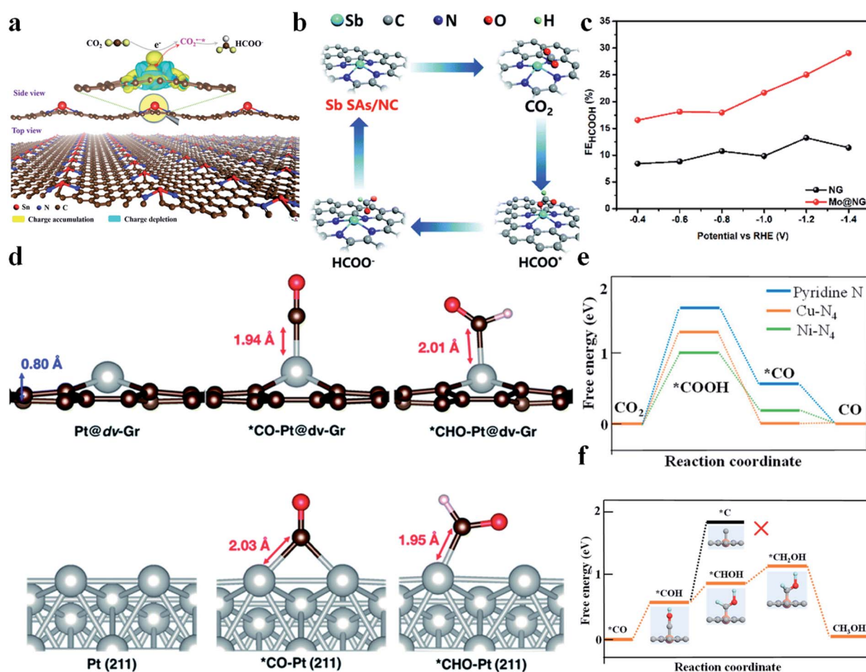
Fig. 9 (a) Plot showing 3D differential charge density of single Sn δ+ atoms on N-doped graphene and the schematic illustration of \text{CO}_2 electroreduction into formate. The yellow and blue isosurfaces correspond to the increase and depletion in the number of electrons, respectively. Reproduced with permission from ref. 99. Copyright (2019) Wiley-VCH. (b) Proposed \text{CO}_2\text{RR} mechanism on Sb SA/NC. Reproduced with permission from ref. 101. Copyright (2020) The Royal Society of Chemistry. (c) Comparison of formate faradaic efficiency between NG and Mo@NG. Reproduced with permission from ref. 102. Copyright (2019) Elsevier. (d) Optimized geometries of Pt@dv-Gr and Pt (211) before and after adsorption of ^*\text{CO} and ^*\text{CHO} . Reproduced with permission from ref. 7. Copyright (2017) The Royal Society of Chemistry. (e) Free energy diagram of \text{CO}_2 reduction to CO on pyridine N, Ni-N 4 , and Cu-N 4 . (f) Free energies for conversion of ^*\text{CO} to \text{CH}_3\text{OH} on Cu-N 4 . Orange, gray, dark blue, red, and light blue spheres stand for Cu, C, N, O, and H atoms, respectively. Reproduced with permission from ref. 105. Copyright (2019) American Chemical Society.
