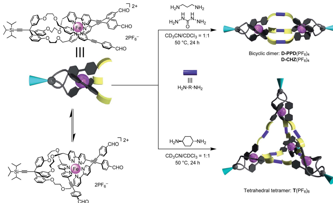
Fig. 6 Bicyclic dimer D-PPD 4+ and D-CHZ 4+ , and tetrahedral tetramer T 8+ , which are constructed by the imine bond formation of [2bFe] 2+ existing as a fac/mer isomeric mixture.
