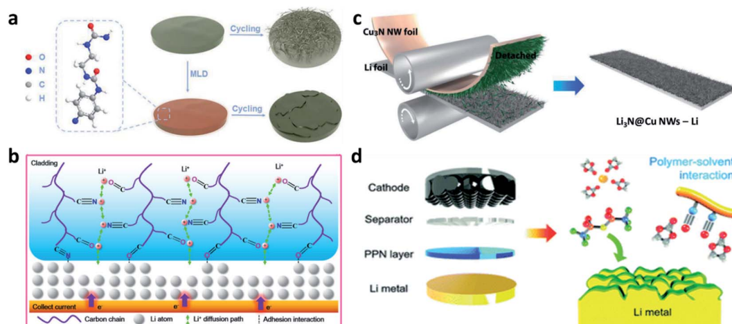
Fig. 2 Constructing artificial SEI layers on Li metal electrodes via physical methods. (a) Schematic illustration of "polyurea" deposited on Li to guide uniform deposition; 65 reproduced with permission. Copyright 2019, John Wiley and Sons. (b) Illustration of P(BMA-AN-St) cladding regulating Li + flux; 66 reproduced with permission. Copyright 2019, American Chemical Society. (c) Fabrication of a Cu 3 N layer on Li foil via physical rolling and printing method; 67 reproduced with permission. Copyright 2020, John Wiley and Sons. (d) Schematic illustration of coating the PPN layer on Li metal in the battery assembly process. 68 Reproduced with permission. Copyright 2019, Royal Society of Chemistry.
