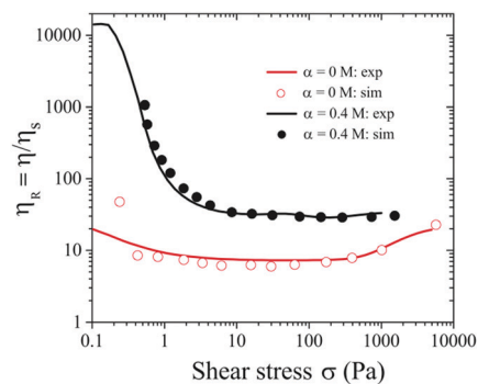
Fig. 7 Relative viscosity ( \eta_R ) versus \sigma for \phi = 0.46 and \alpha = 0 and 0.4 M . Symbols represent numerical data at \alpha = 0 and 0.4 M respectively, and solid lines represent experimental data.
