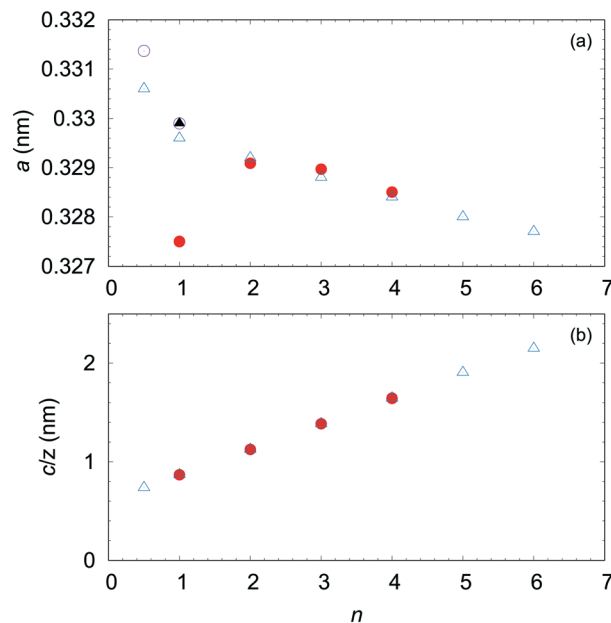
Fig. 18 (a) Lattice parameter a and (b) layer width c / Z of homologous compounds InGaO 3 (ZnO) n as function of n . Open triangle symbols represent lattice constants estimated from the polycrystalline sample. 23 Solid triangles represent small single crystal obtained from high pressure (2 GPa). 45 Open circle symbols represent estimates from single crystals grown by the OFZ method. 55 Solid circles represent estimates from small single crystals. 46,48,49
