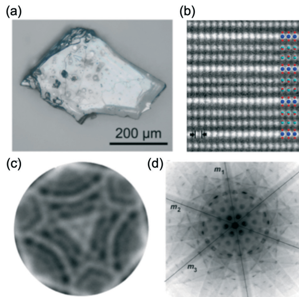
Fig. 4 (a) Optical micrograph image of a single crystal of \text{InGaO}_3(\text{ZnO})_{11} . (b) HAADF image of \text{InGaO}_3(\text{ZnO})_{11} in [1\bar{1}00] orientation with structure model. The blue, red, and light green circles represent In, Zn/Ga, and O atoms, respectively. Cation columns of In (bright) and Zn/Ga (medium bright) are well resolved indicating the cation layer stacking in \text{InGaO}_3(\text{ZnO})_{11} . A spacing of 0.16495 nm of the (2\bar{1}\bar{1}0) prism planes is shown. (c) Central CBED disc and (d) whole pattern results suggest 3m symmetry. Panels (a-d) are reprinted with permission from ref. 46. © 2014 Elsevier.
