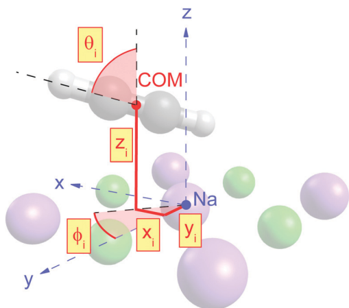
Fig. 4 Illustration of the molecular structure parameters of a molecule M_i adsorbed over a sodium Na. The parameters x_i , y_i , and z_i represent the local position of the center of mass (COM, red point) relative to the sodium (blue point). The azimuthal orientation \phi_i is measured against the y -axis, the tilt angle \theta_i is measured against the surface normal.
