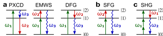
Fig. 8 Diagrams for various nonlinear enantio-sensitive or chiral-sensitive processes. Different colors mark different directions of light polarization (e.g. green – x , red – y , blue – z ). Straight up and down arrows indicate photon absorption and photon emission, wavy arrows indicate induced polarization. (a) Diagrams for photo-excitation circular dichroism (PXCD), enantio-sensitive microwave spectroscopy (EMWS), and difference-frequency generation (DFG); (b) sum-frequency generation (SFG). For SFG, the field pseudovector is given by \vec{L} = \vec{E}(\omega_1) \times \vec{E}(\omega_2) 44,139 and thus it vanishes when \omega_1 = \omega_2 , i.e. second harmonic generation requires more than two photons. (c) Second harmonic generation (SHG) is indeed possible for higher-order processes because these are associated with field pseudovectors such as \vec{L} = [\vec{E}(\omega_1) \cdot \vec{E}(\omega_1)] [\vec{E}^*(\omega_1) \times \vec{E}(\omega_1)] , which are non-zero for elliptically polarized light and record its rotation direction.
