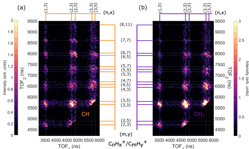
Fig. 10 Zoomed in AEPICOP of ion pairs recorded in coincidence with CH AES band (a) and CH 2 AES band (b) following ionization of adamantane at h\nu = 350 eV. The maps have been normalized to maintain the 4 : 6 (4CH : 6CH 2 ) ratio that we expect in the adamantane molecule.
