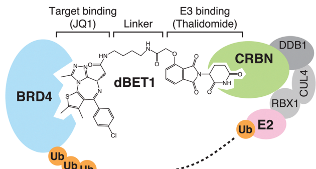
Fig. 11 CRBN-based PROTACs. dBET1, one of the CRBN-based PROTACs, consists of a linker connecting thalidomide and JQ1, the latter of which binds to its target BRD4. Formation of the ternary complex shown in the figure leads to the degradation of BRD4 via CRL4 CRBN .
