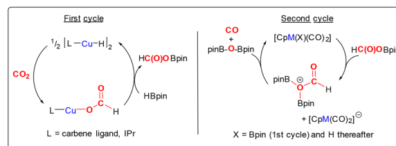
Scheme 43 Mechanism for the 2-electron reduction of CO 2 to CO catalysed by heterobimetallic complexes [(NHC)Cu–ML n ] {ML n = [FeCp(CO) 2 ], [WCp(CO) 3 ], [MoCp(CO) 3 ]}. © The Royal Society of Chemistry 2022
