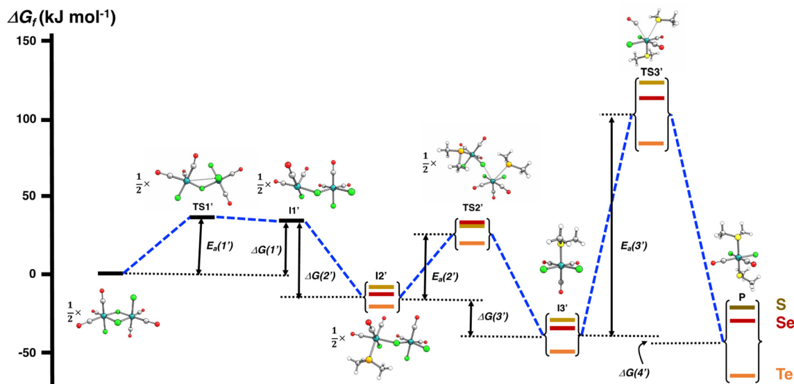
Fig. 5 PBE0-D3/def2-TZVP energy profile of the reaction of [\text{RuCl}_2(\text{CO})_3]_2 and \text{EMe}_2 ( E = \text{S, Se, Te} ) in \text{CH}_2\text{Cl}_2 .
