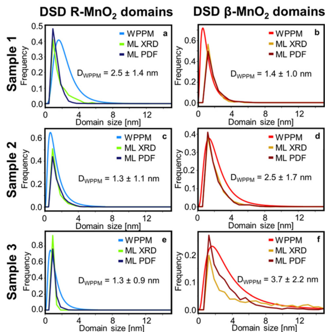
Fig. 8 Domain Size Distributions (DSD) determined by Whole Powder Pattern Modelling (WPPM), ML-MotEx analysis of XRD (ML XRD) and PDF (ML PDF) refinement results of R- and \beta - MnO_2 domains in samples 1 (a and b), 2 (c and d) and 3 (e and f).
