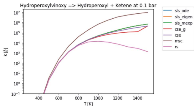
Fig. 7 Rate coefficient for hydroperoxyl + ketene at 0.1 bar.
