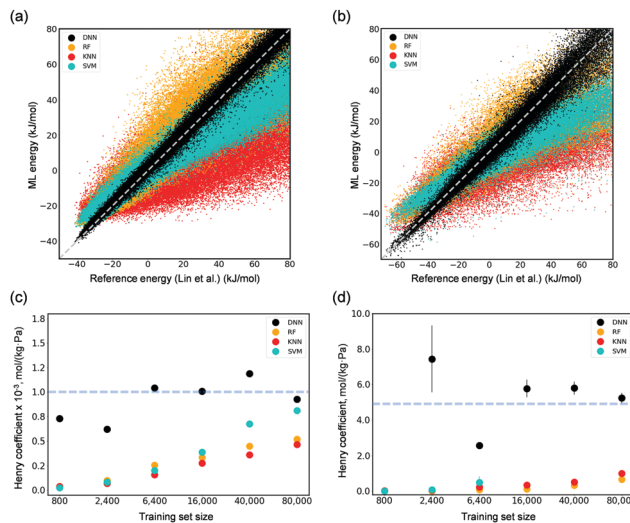
Fig. 2 Parity plots of the ML-predicted (DNN, RF, KNN, and SVM) energies and reference values computed by the force field of Lin et al. 5 for 0.4 M unseen points regarding (a) \text{CO}_2 adsorption and (b) \text{H}_2\text{O} adsorption in Mg-MOF-74. Calculated Henry's coefficients of (c) \text{CO}_2 and (d) \text{H}_2\text{O} adsorbed in Mg-MOF-74 as a function of the training size from as small as 800 to as large as 80 000. The dotted lines in (c) and (d) represent the reference value ( i.e. , \sim 1.0 \times 10^{-3} mol ( \text{kg}^{-1} \text{Pa}^{-1} ) for \text{CO}_2 and \sim 5 mol ( \text{kg}^{-1} \text{Pa}^{-1} ) for \text{H}_2\text{O} ) computed by the force field of Lin et al.
